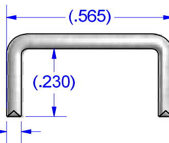
BUSS #14257 COPPER (TIN SOLDERABLE)
