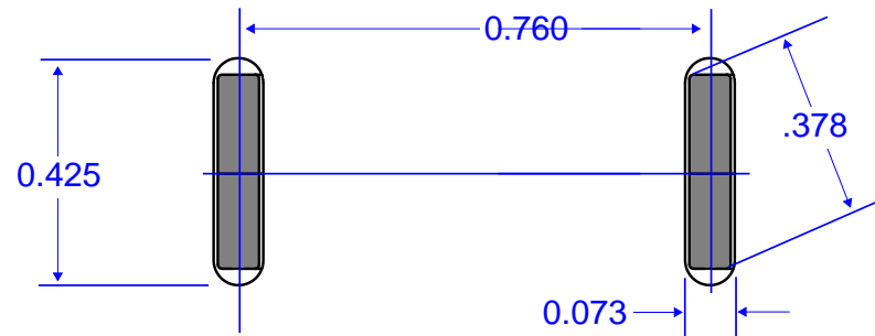
NOMINAL PCB SLOT CUTOUTS
