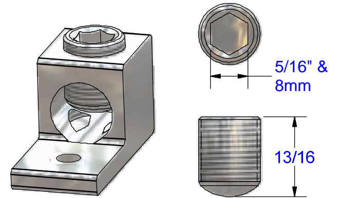
SCREW #14237M Tin Plated Aluminum
